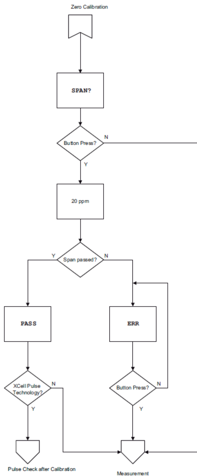
Figure 12 Span calibration
