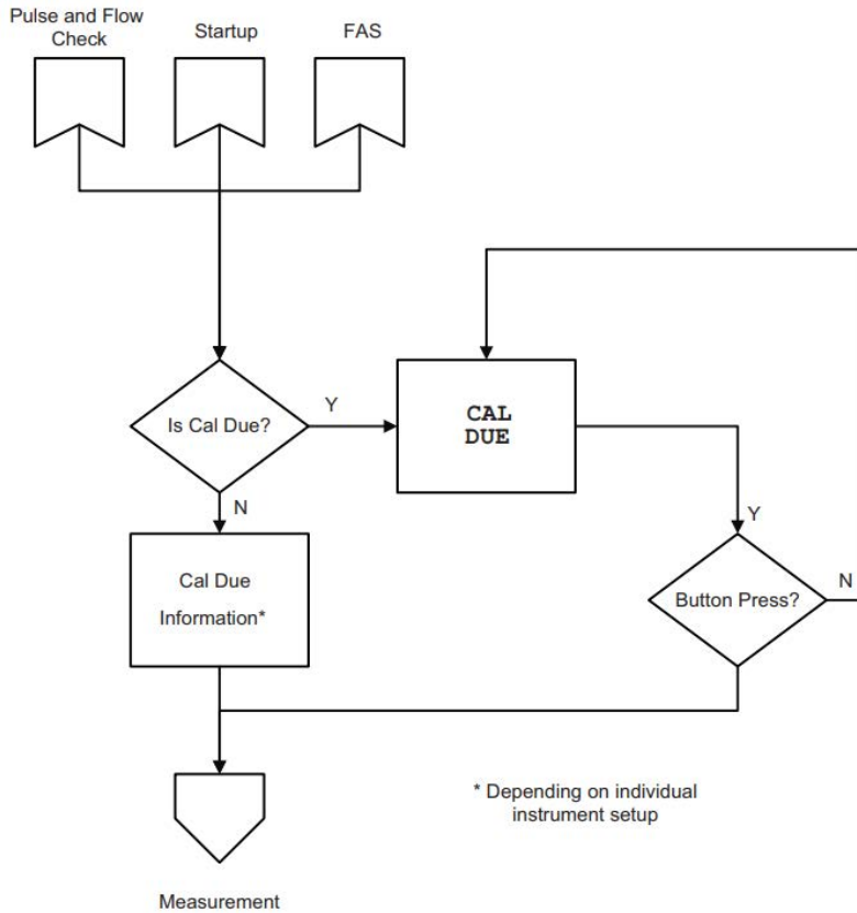
Figure 7 Calibration due
