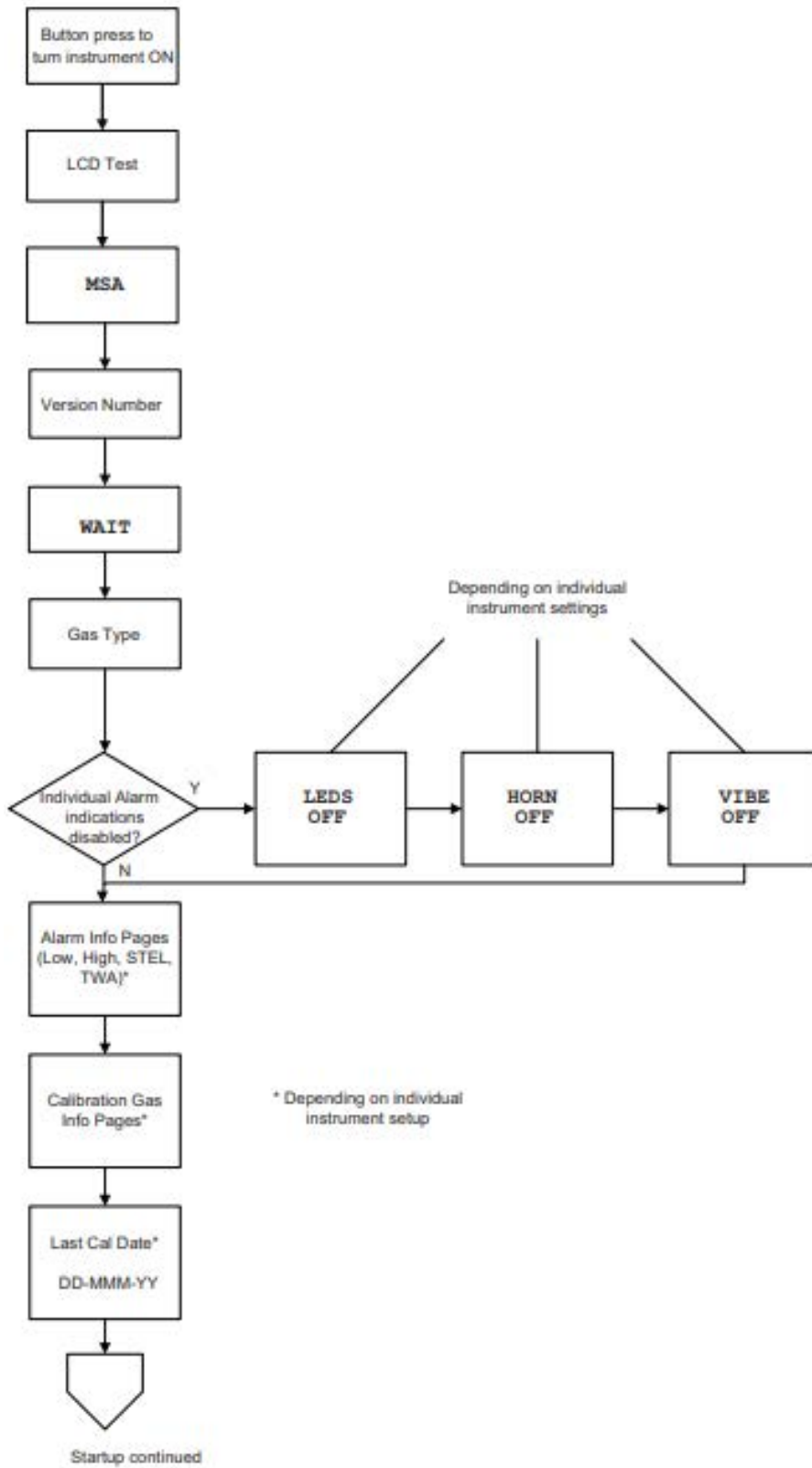
Figure 3 Startup
